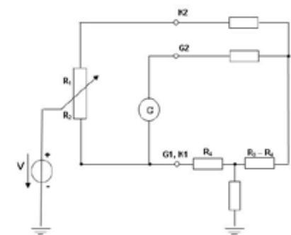
➤ Glaser – Measuring Circuit, ground related voltage source
