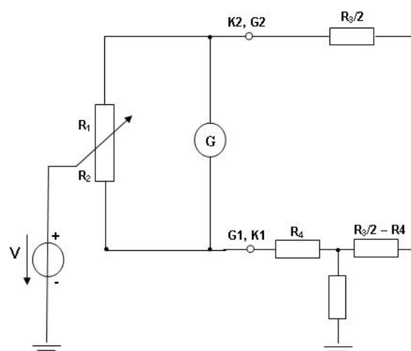
➤ Murray – Measuring Circuit
