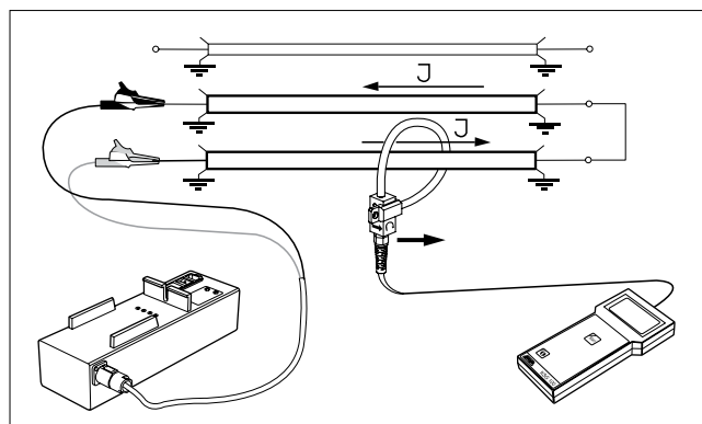
➤ galvanic connection on single core cables, off-line connection
