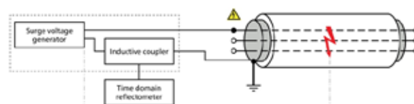
➤ schematic connection for ICM
