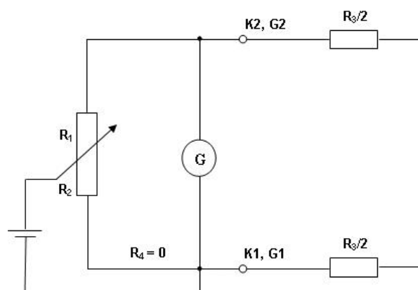
➤ Murray – Balancing Circuit
