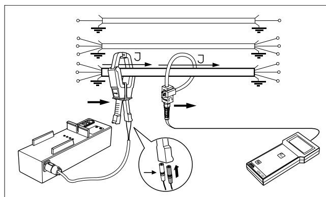
➤ inductive connection to live cable via CT clamp AZ10
